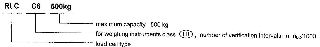
Figure 1: Load cells type RLC C6 0,5t and type RLC C3 28t
